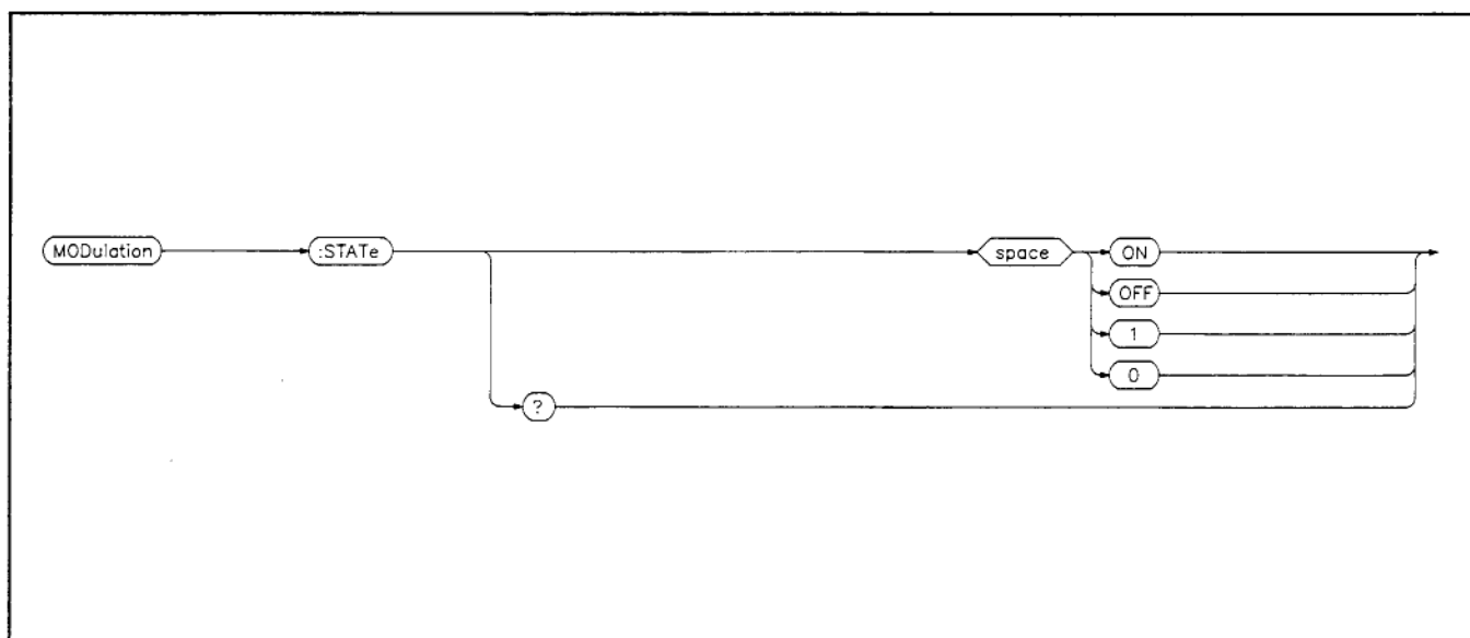
Figure 6-17. Modulation Subsystem.
