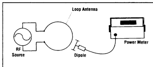
Figure 11. Absolute measurement loss — loop antenna to dipole antenna
