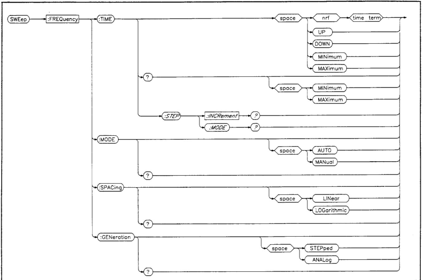
Figure 6-25. Sweep Subsystem.
