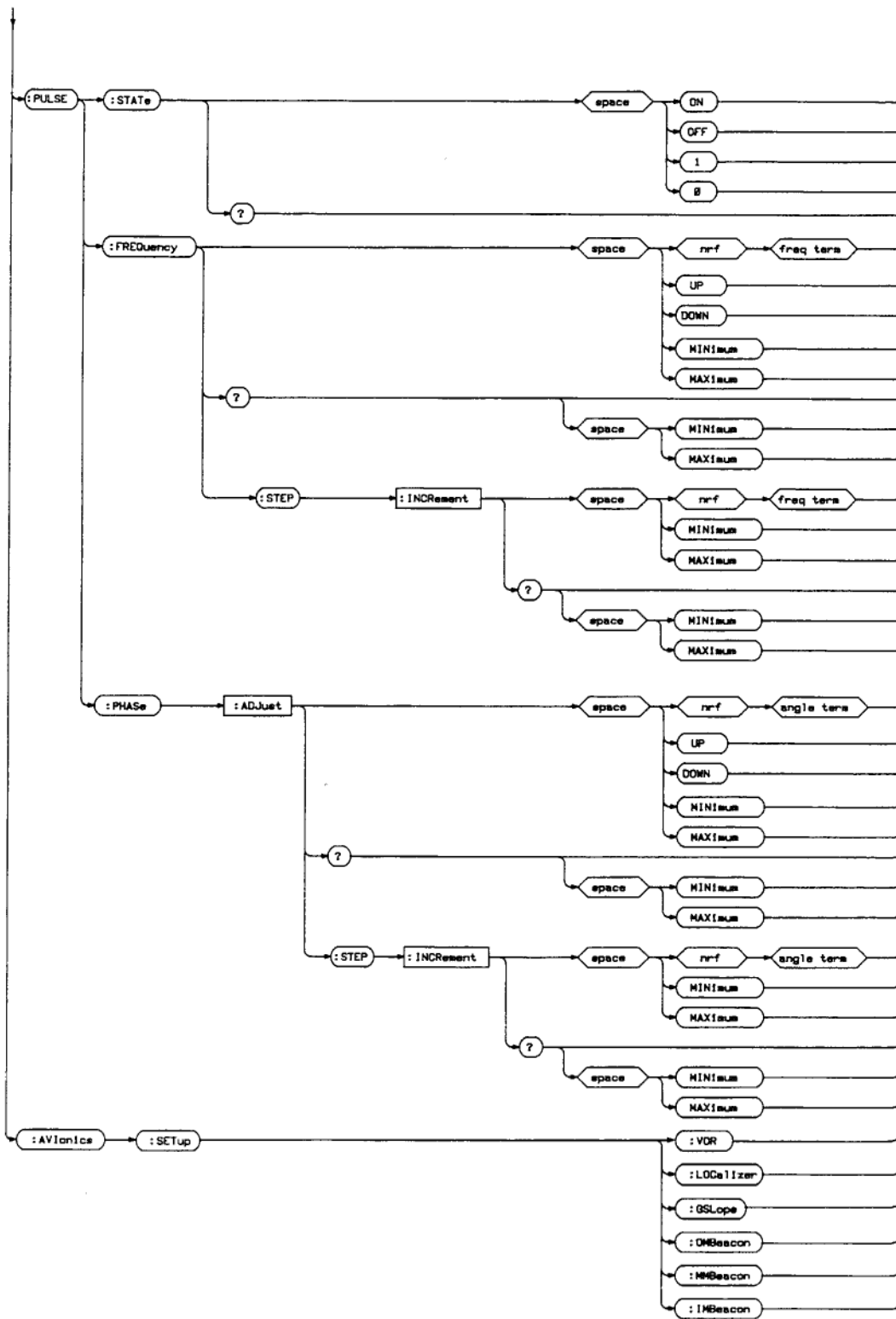
Figure 6-15. LF Source Subsystem. (6 of 6)
