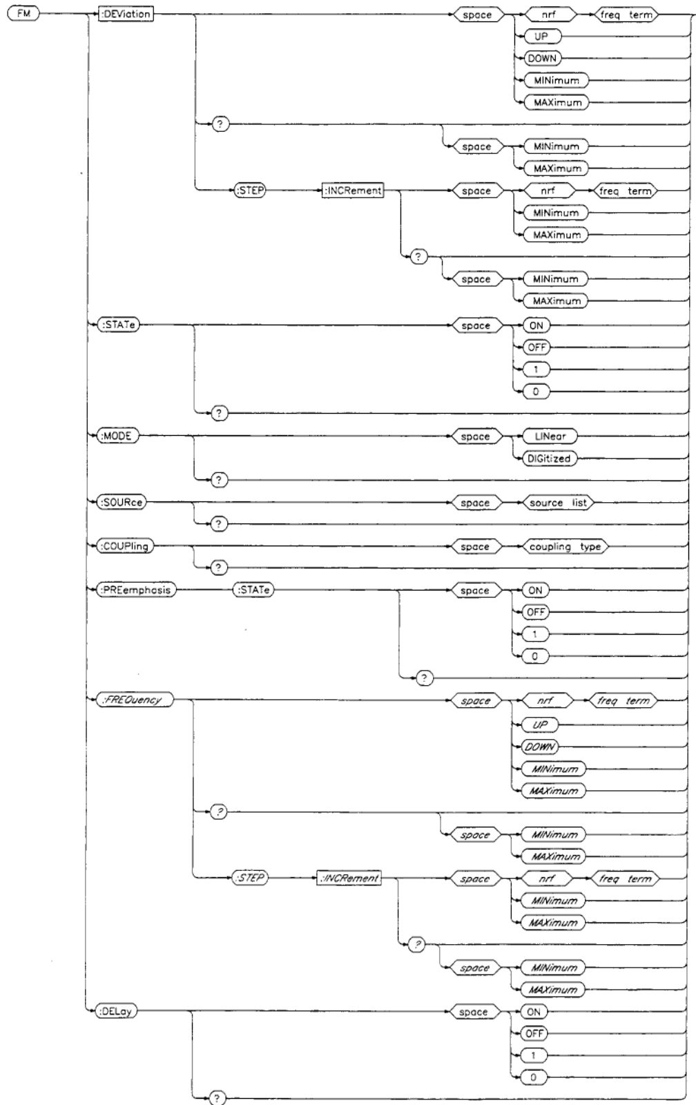
Figure 6-9. FM Subsystem.
