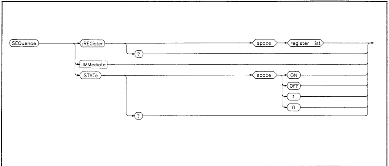
Figure 6-23. Sequence Subsystem.
