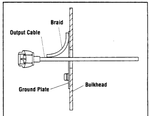
Figure 16. RF leakage wire passage option 10
