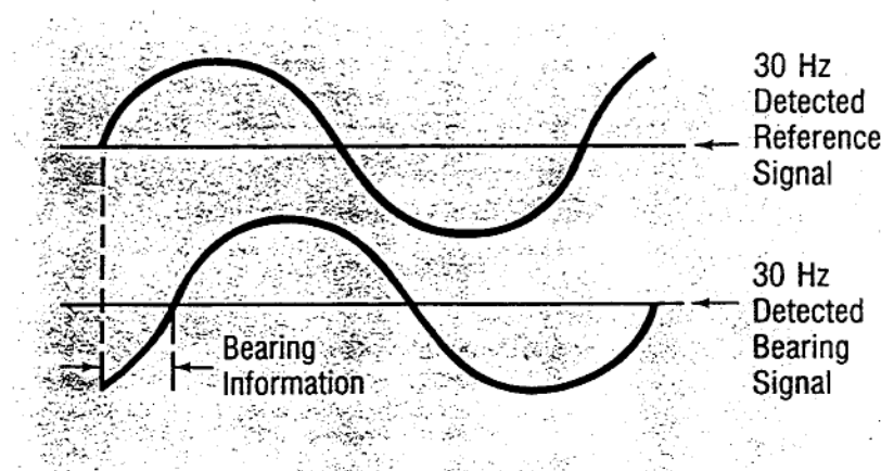
VOR Signal Seen at Aircraft Receiver
