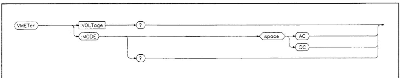
Figure 6-27. Voltmeter Subsystem.
