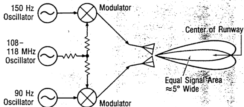
Localizer Transmitter System and Antenna Pattern.
