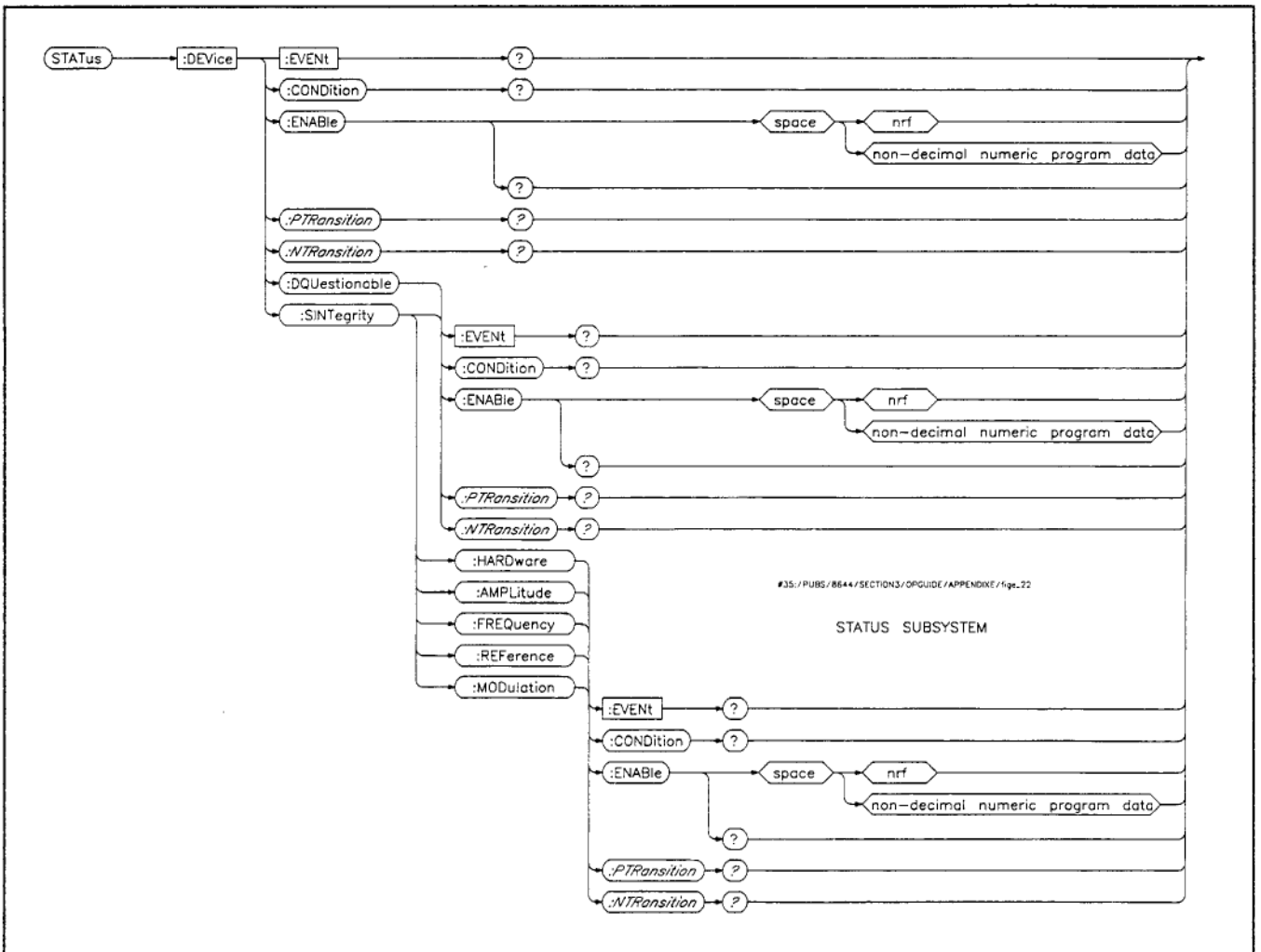
Figure 6-24. Status Subsystem.
