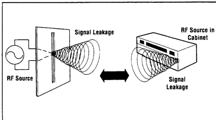
Figure 13. Simulation equivalents to signal generator cabinet
