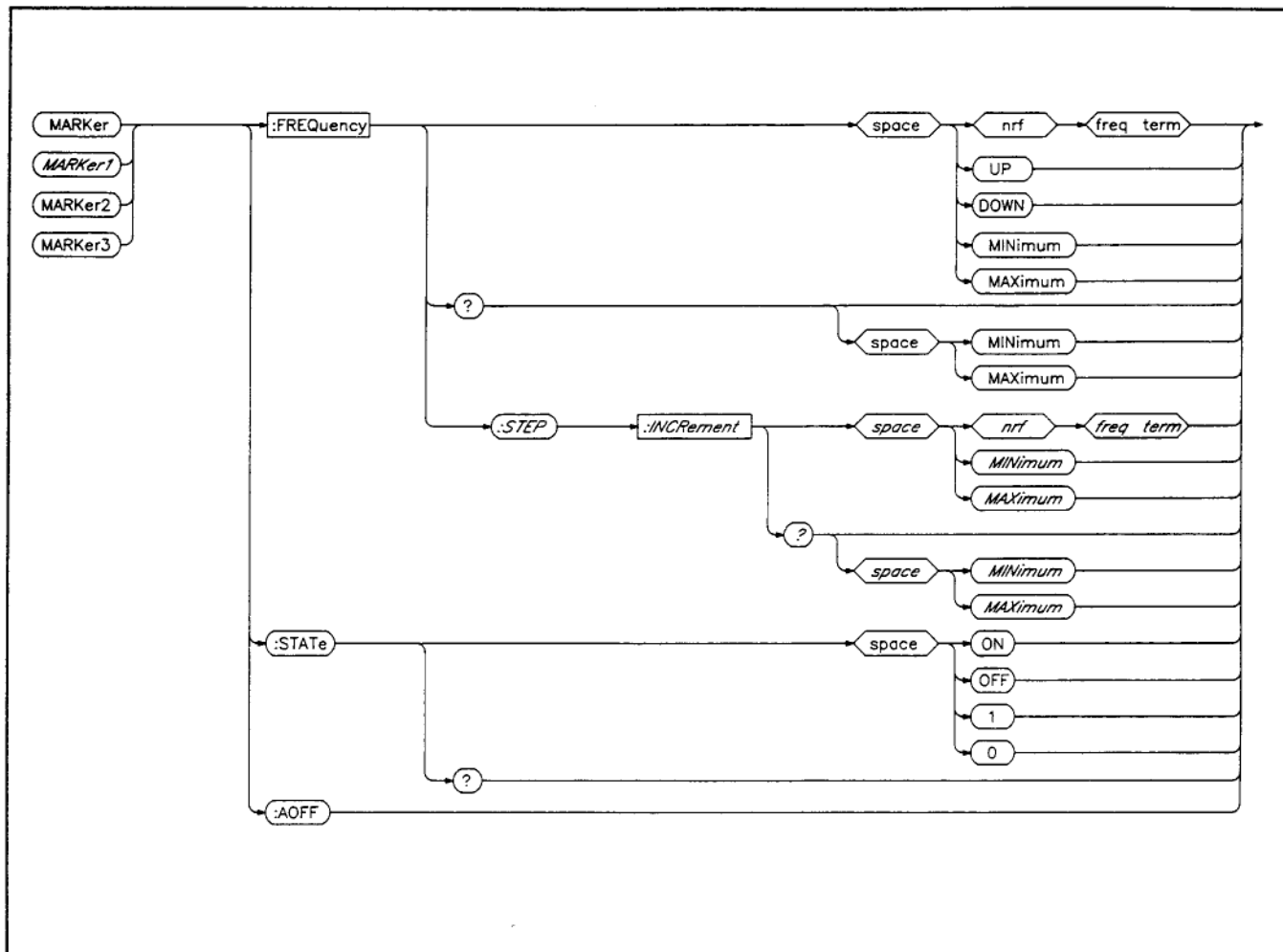
Figure 6-16. Marker Subsystem.
