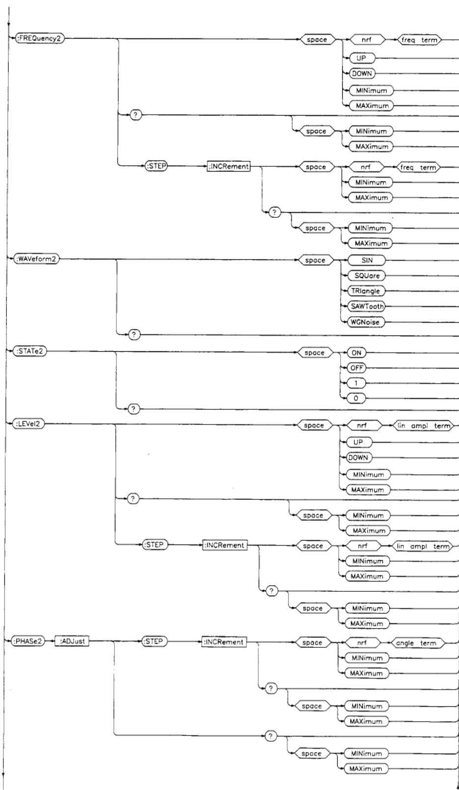
Figure 6-15. LF Source Subsystem. (2 of 6)
