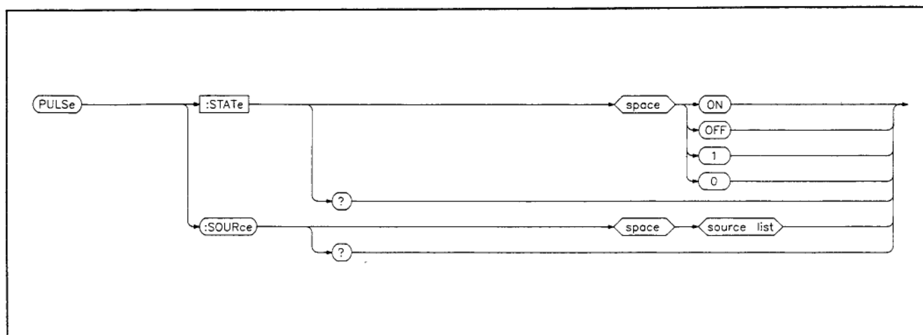
Figure 6-21. Pulse Subsystem.
