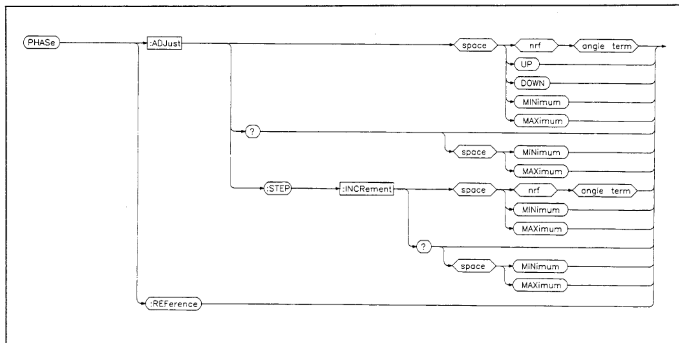
Figure 6-19. Phase Subsystem.
