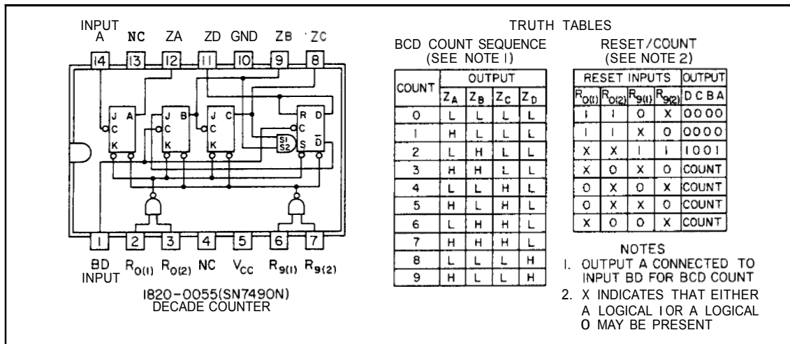
Figure 4-4. Decade Counter 1820-0055
