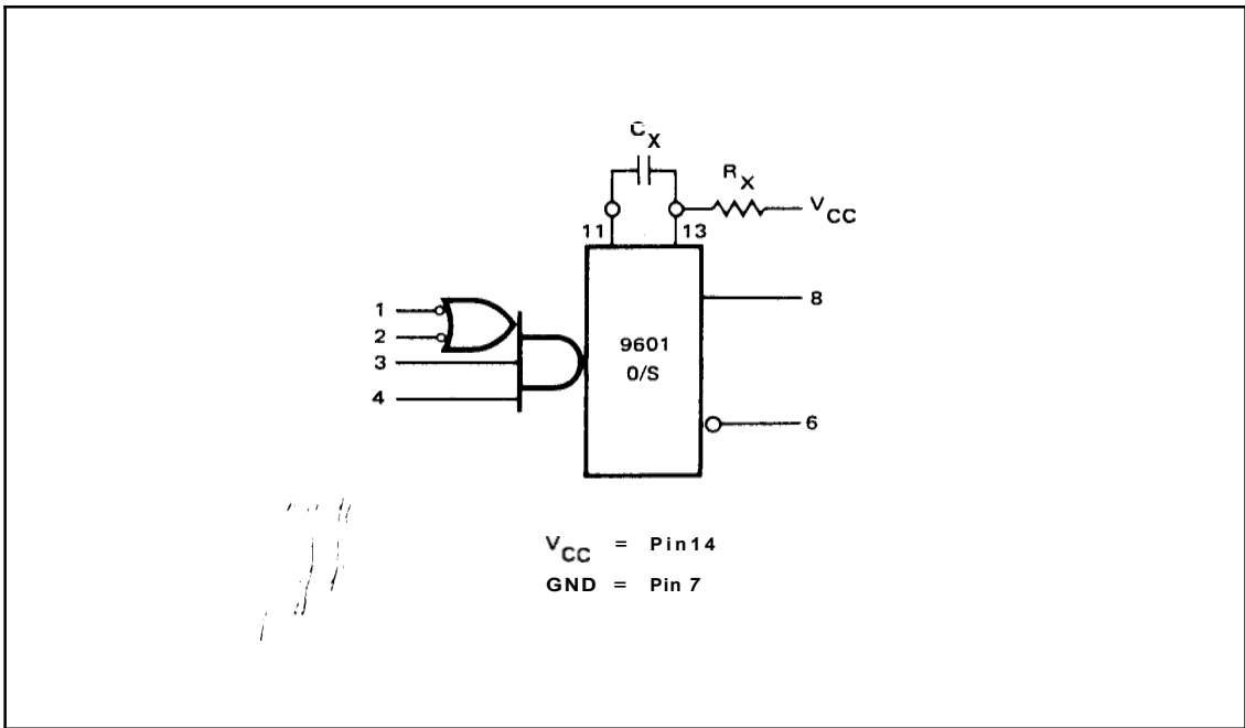
Figure 4-8. Monostable Multivibrator 1820-0207
