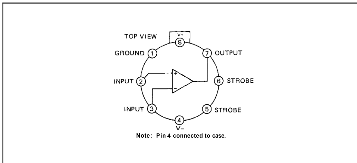
Figure 4-15. Voltage Comparator/Buffer 1820-0475
