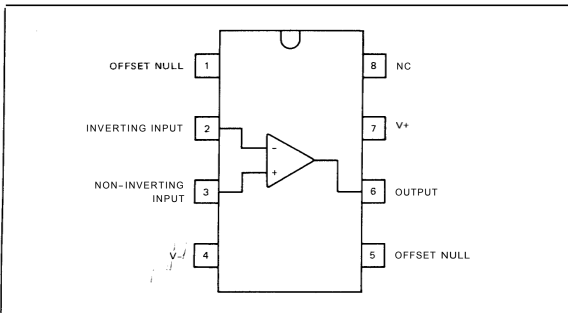
Figure 4-42. Operational Amplifier 1826-0073
