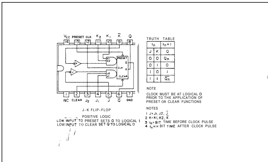
Figure 4-5. J-K Flip-Flop 1820-0065
