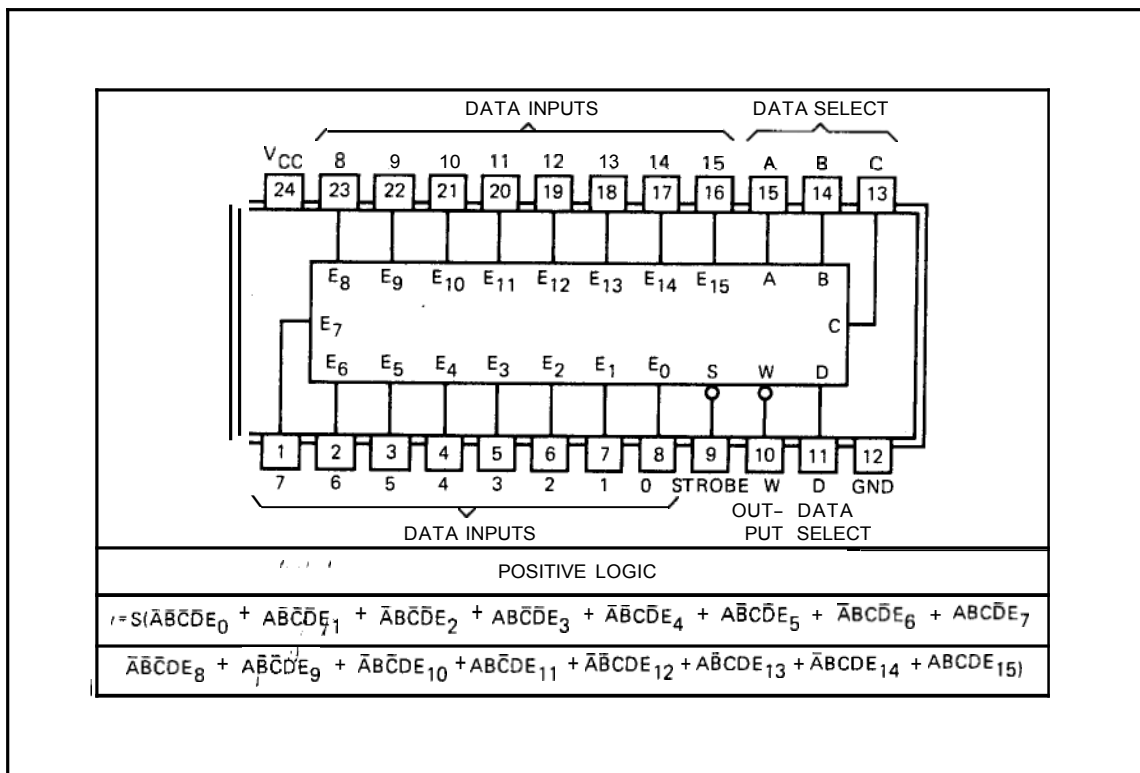
Figure 4-25. Data Selectors/Multiplexers 1820-0640
