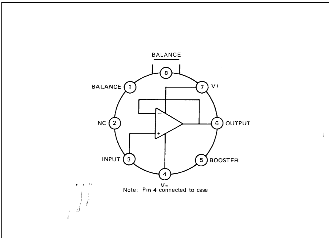
Figure 4-40. Operational Amplifier 1826-0021
