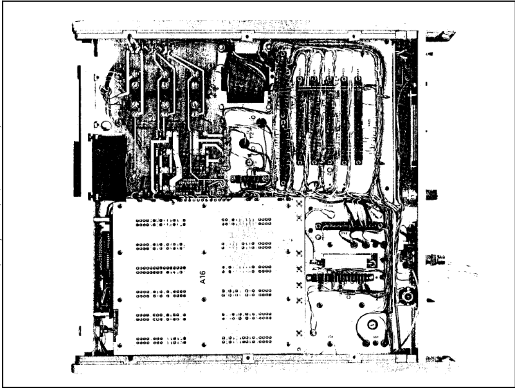
Figure 8-3. 5540A Bottom Internal View and Cable Numbers and Connections (with Options 001, 002, and 011 Installed)
