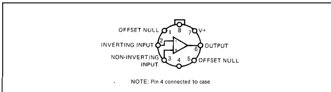
Figure 4-10. Operational Amplifier 1820-0216
