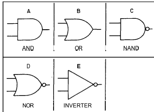
Figure 4-2. Gate Symbols
