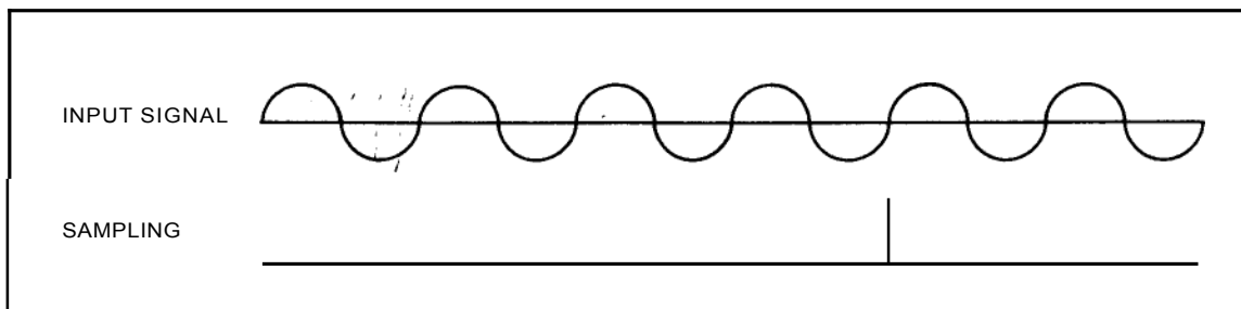
Figure 4-49. Sampling Timing
