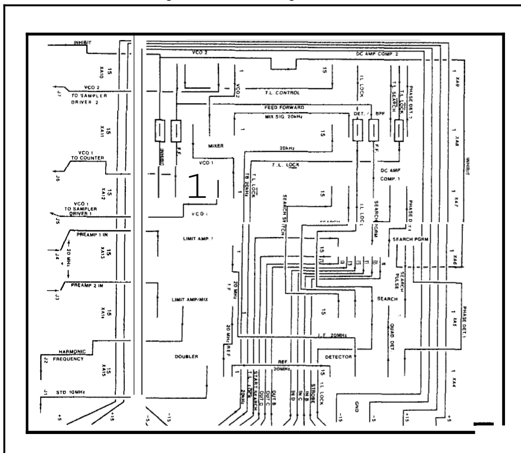
Figure 8-22. A16 Casting Motherboard
