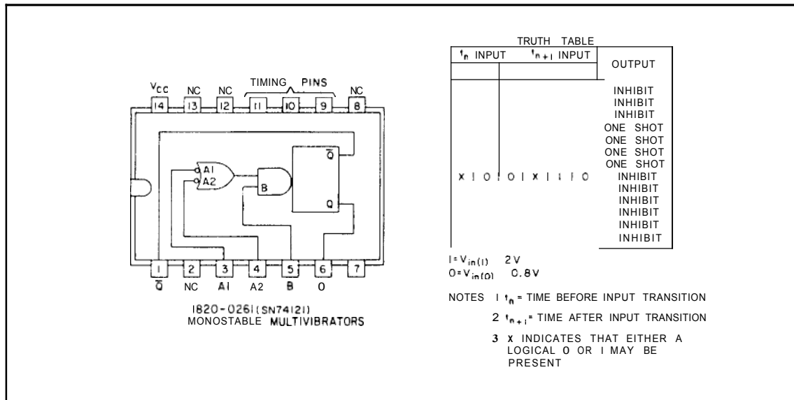
Figure 4-11. Monostable Multivibrator 1820-0261
