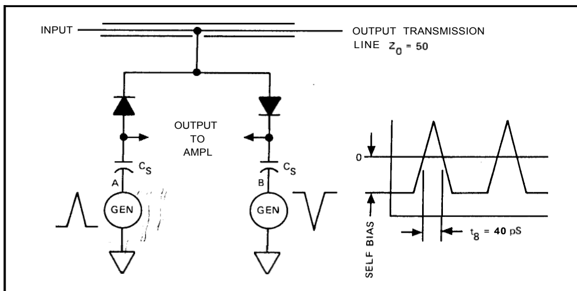
Figure 4-47. Balanced Sampler
