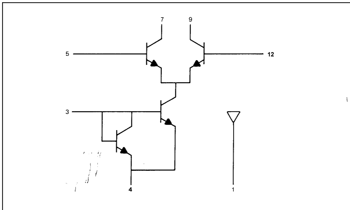
Figure 4-44. Transistor Array 1858-0018
