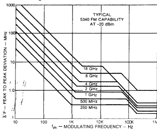
Figure 3-1. FM Characteristics
