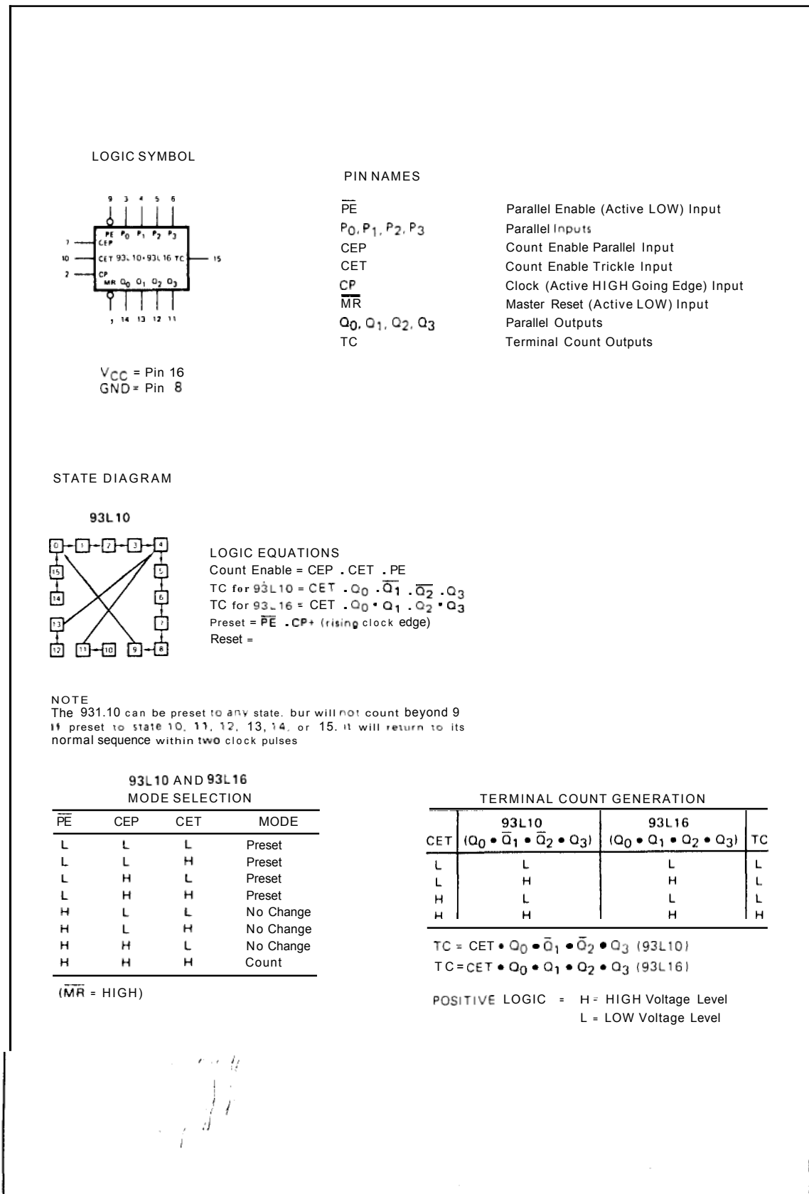
Figure 4-28. Low-Power BCD Decade Counter 1820-0669
