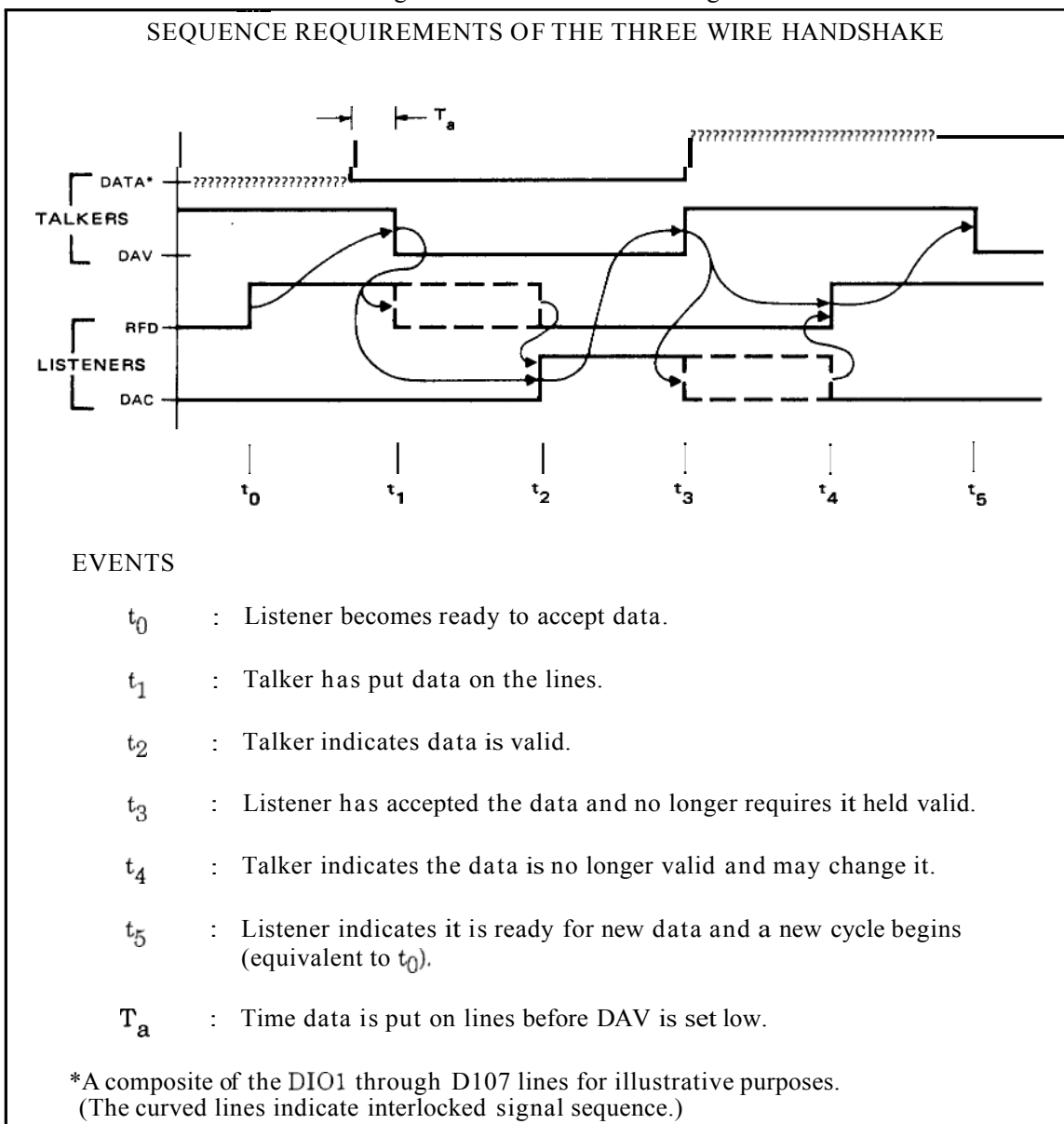
Figure 2-1. Handshake Timing
