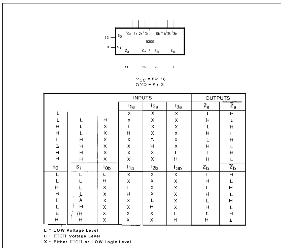
Figure 4-22. Four-Input Multiplexer 1820-0610
