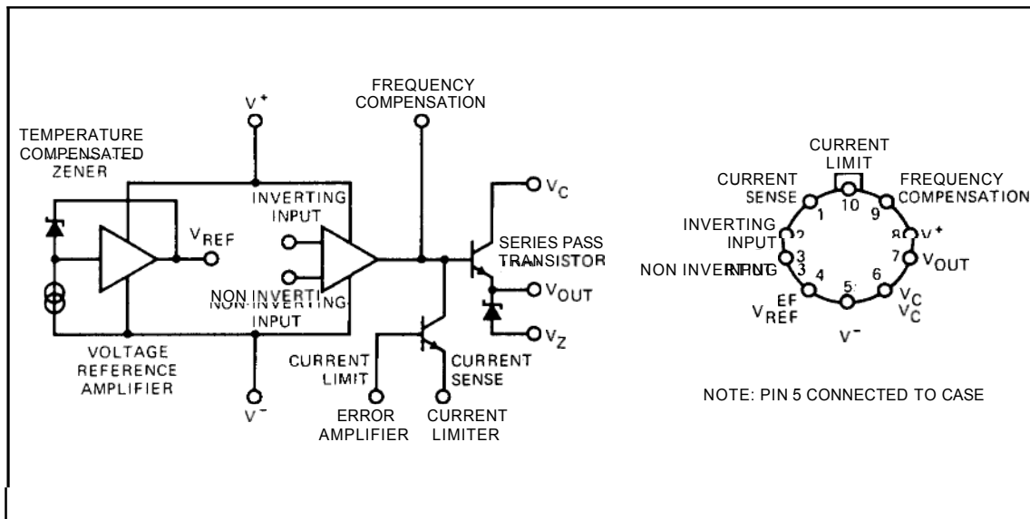
Figure 4-38. Voltage Regulator 1826-0010
