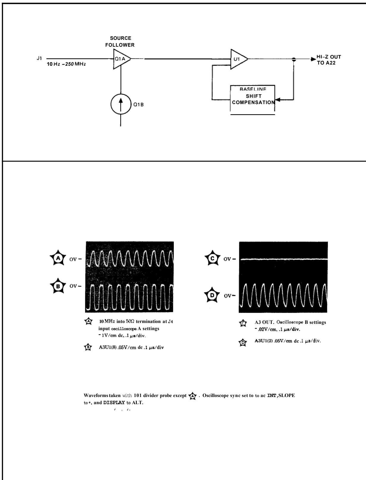
Part of Figure 8-9. A3 HI-Z Input Amplifier Assembly
